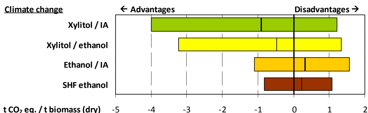
Fig. 5-1 Environmental impacts of production and use of various biorefinery products from wheat straw. Exemplary net results are shown per tonne of biomass input (dry matter) in the category climate change. The coloured bars show the bandwidths of results under favourable and less favourable conditions and the black lines show the results under standard conditions.
